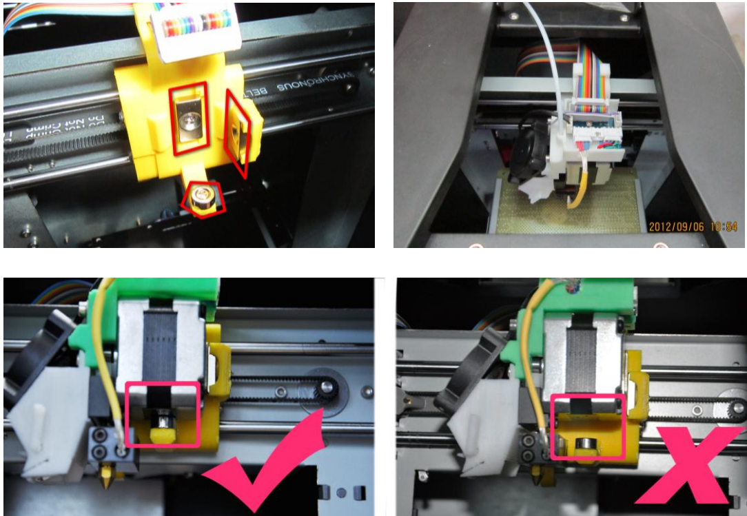
Figure6. Print head installation
