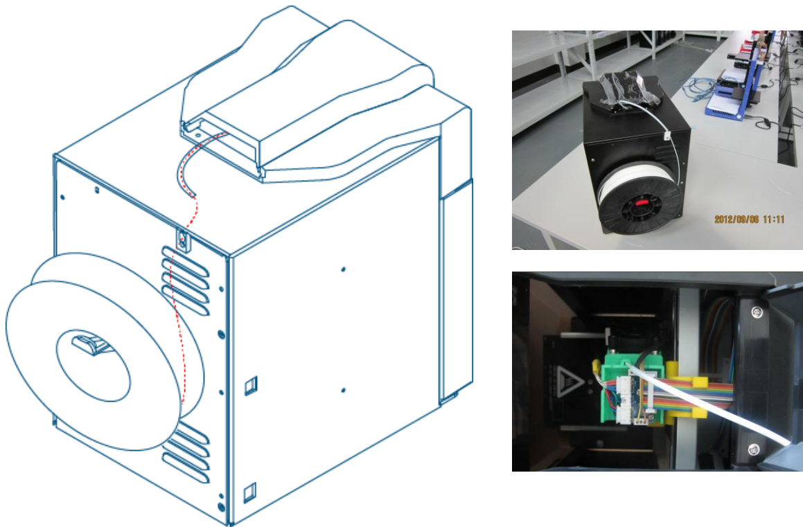
Figure 9. Material Wiring
