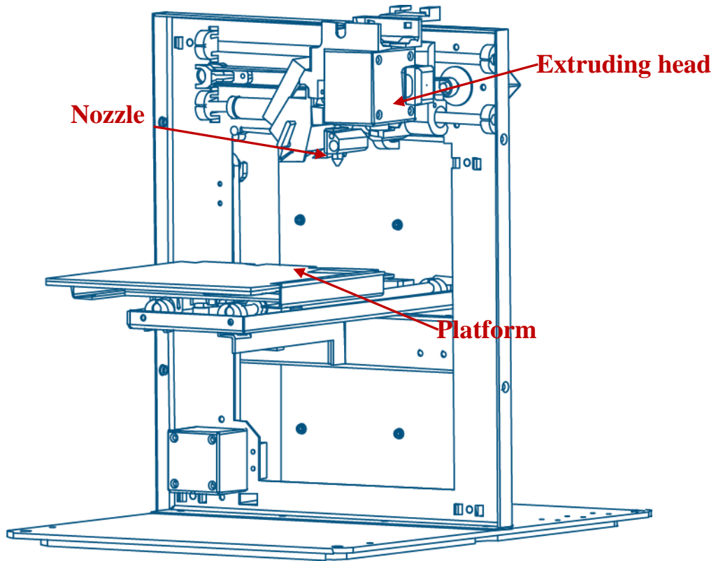
Figure 2. Inside View of UP! mini
